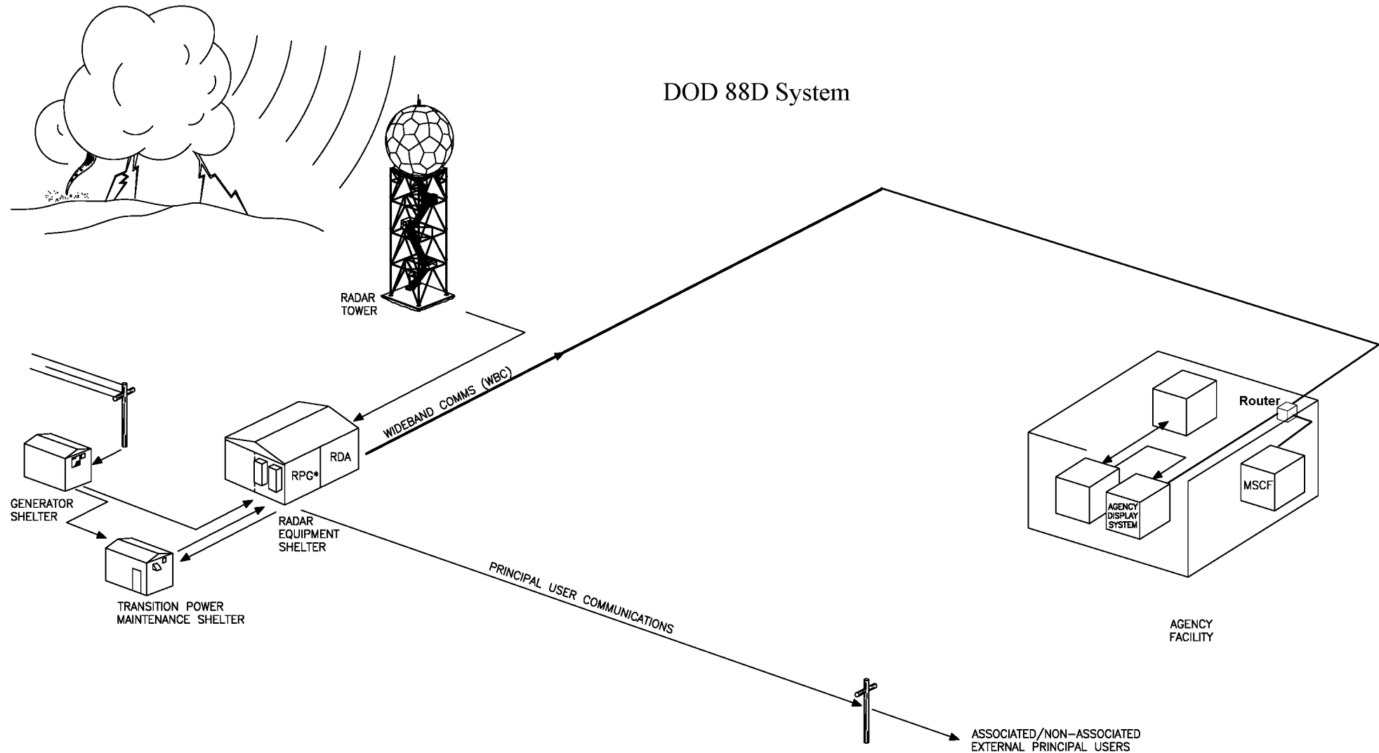
Based on the following drawing Figure FO1-1. Doppler Meteorological Radar WSR-88D, Pictorial Overview
