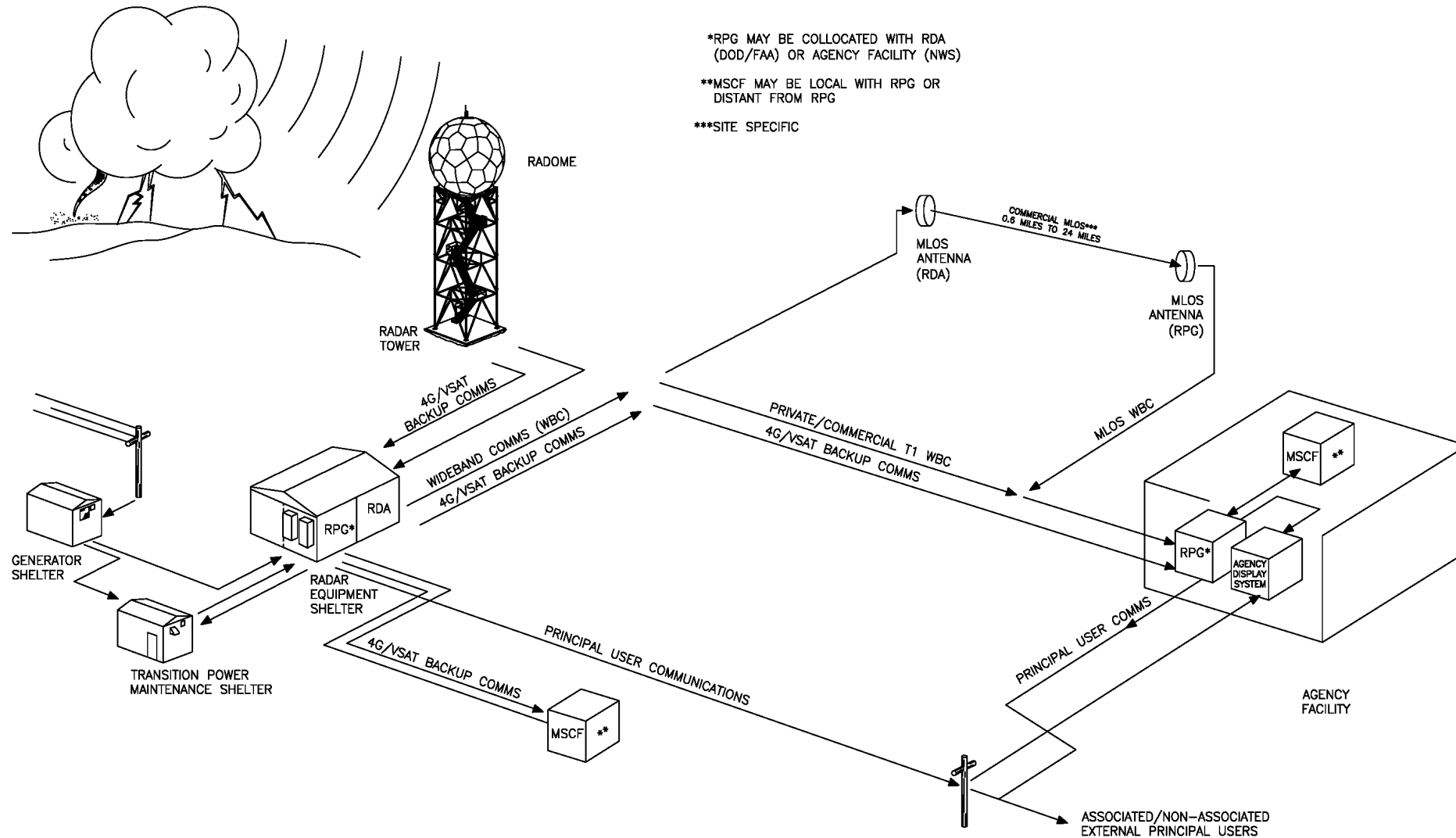
Figure FO1-1. Doppler Meteorological Radar WSR-88D, Pictorial Overview
